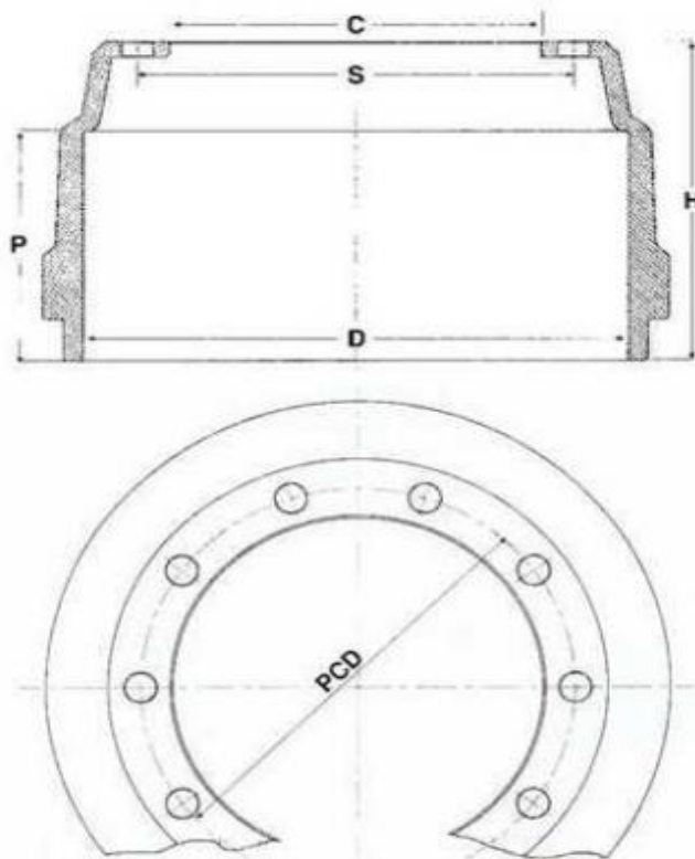
Drum Dimensions
